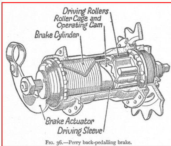
FIG. 36.—Perry back-pedalling brake.
