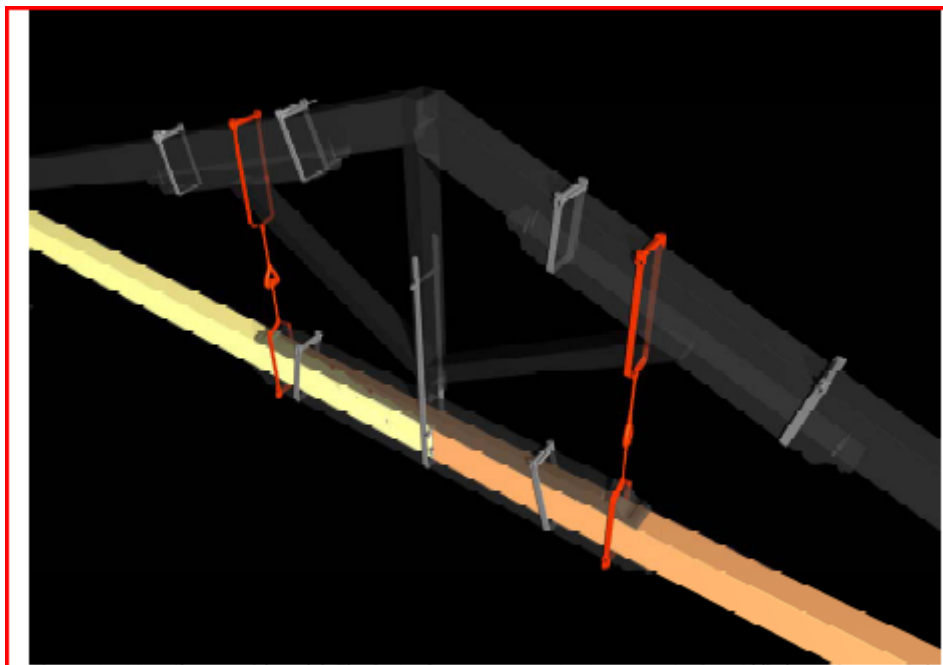
Figure 11. Vasari's truss, 3d model. The Jupiter's arrow connection is not put in the middle but sideways. Only by means of the two iron suspenders (red in the figure), placed in the first half of the XIX c., prevent from rotation the two stumps of the chord
