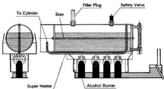
Fig.2 : Pot Type Boiler As Used on the ASTER GER 0-6-OT
