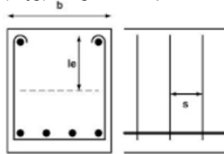
Rectangular Beam - Stirrups
